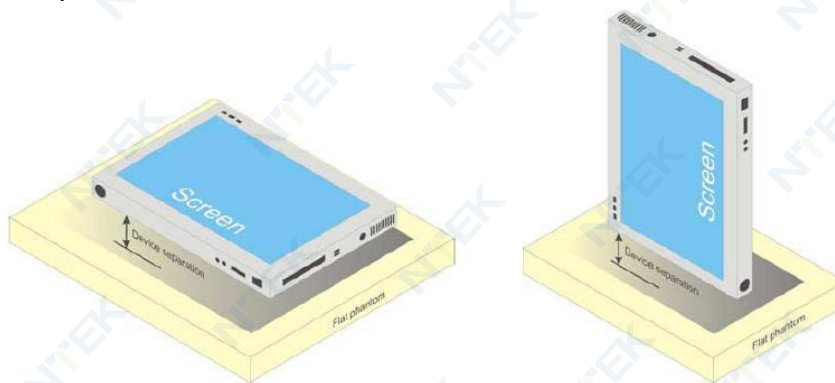
Figure 6.1 – Test positions for Body-supported device
