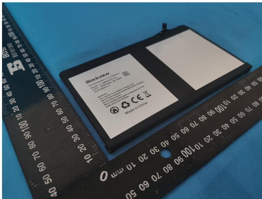
Rechargeable Li-ion Battery Model: Li 398091HTT-B 3.87V 22000mAh 85.14Wh 1ICP4/80/91-4
