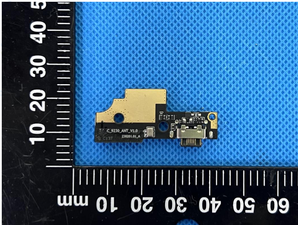
Fig. 11 PCB view
