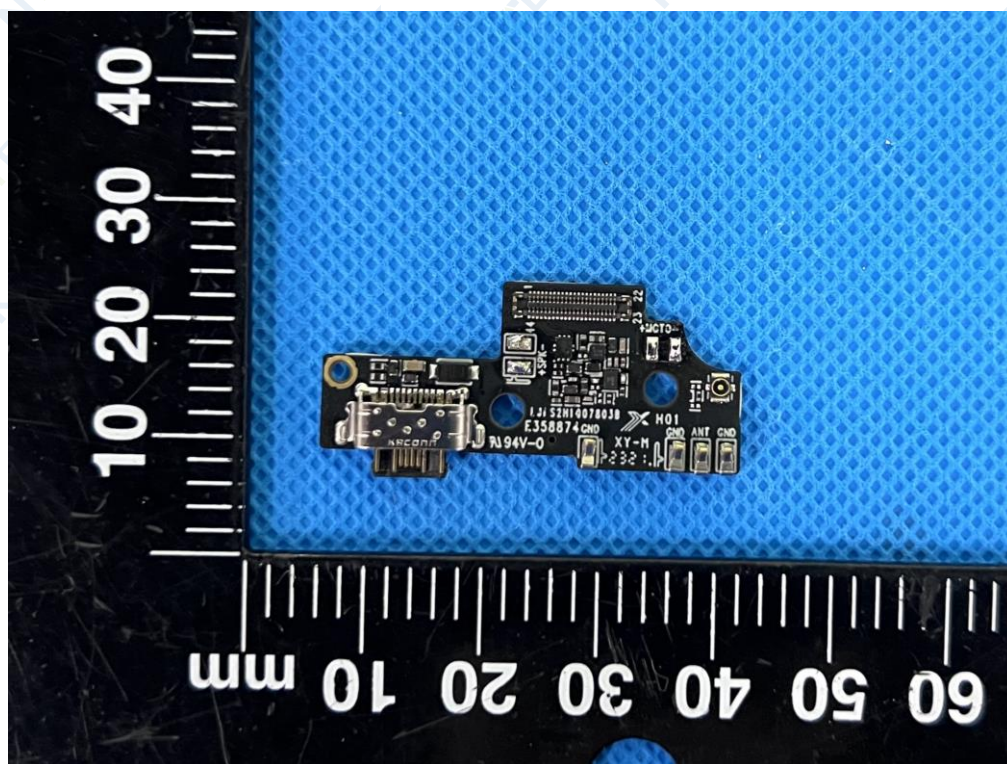
Fig. 10 PCB view
