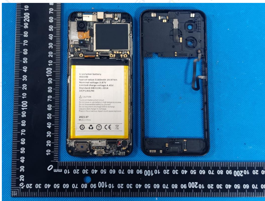
Fig. 7 Internal view
