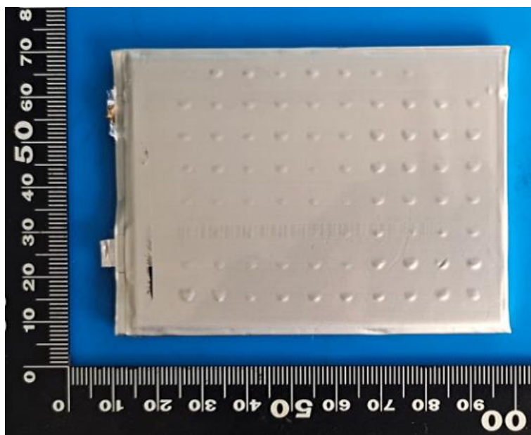
Fig. 3 – Front view of Cell 表3 –电芯正面视图
