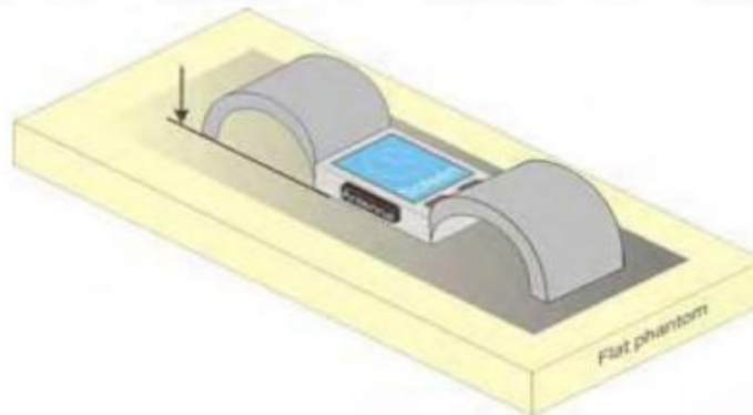
Figure1 Test position for limb-worn devices
