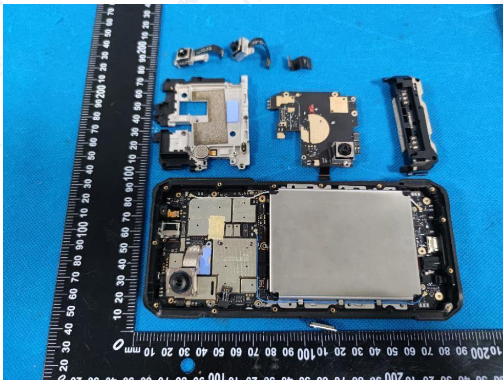
Fig. 8 internal view
