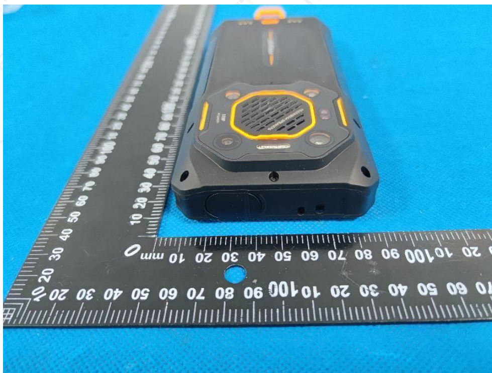
Fig. 5 external view
