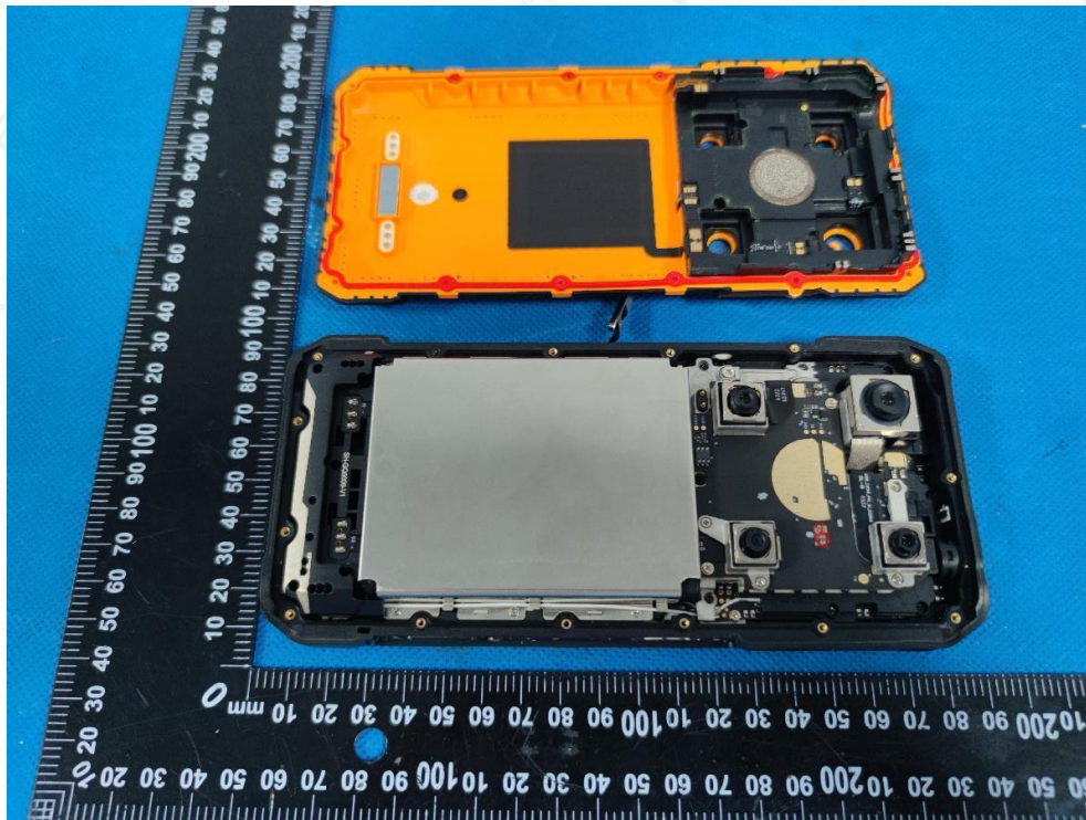
Fig. 7 internal view
