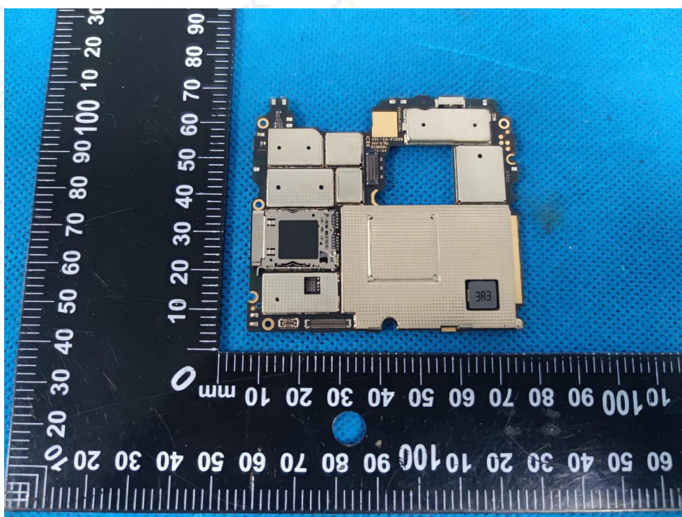
Fig.14 PCB view
