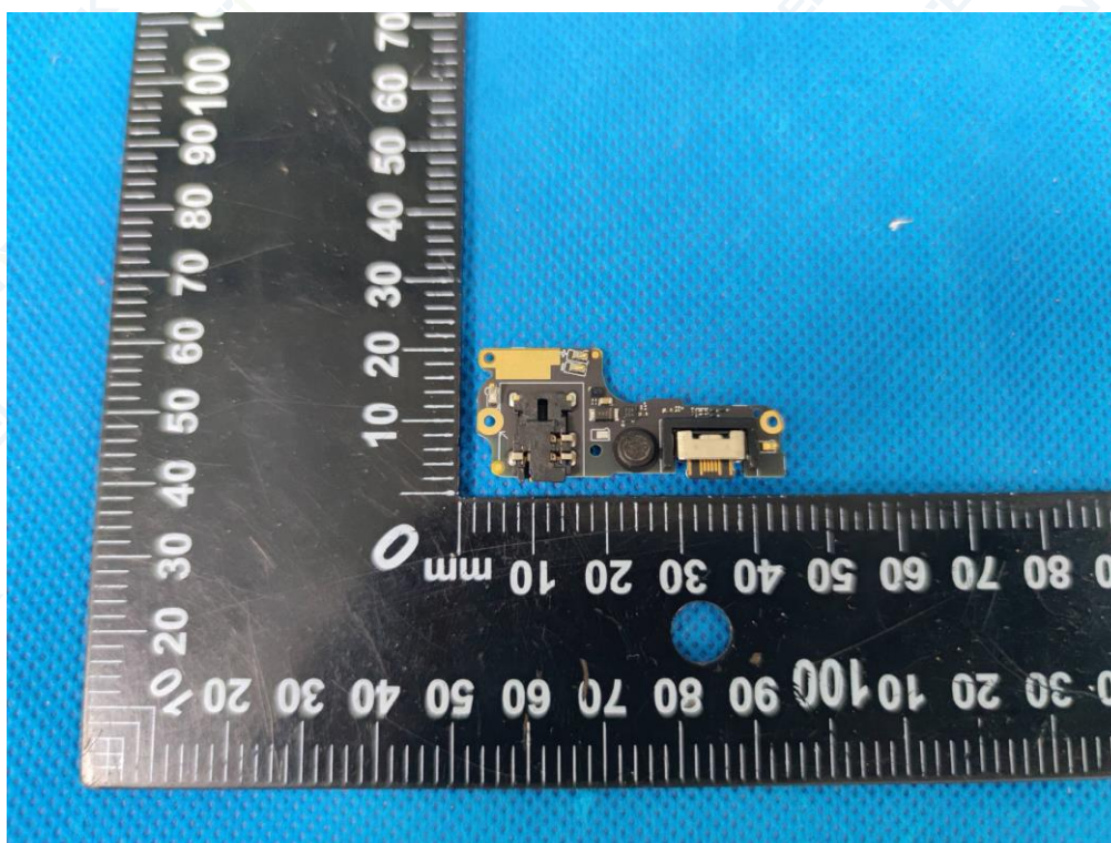
Figure 12 PCB view
