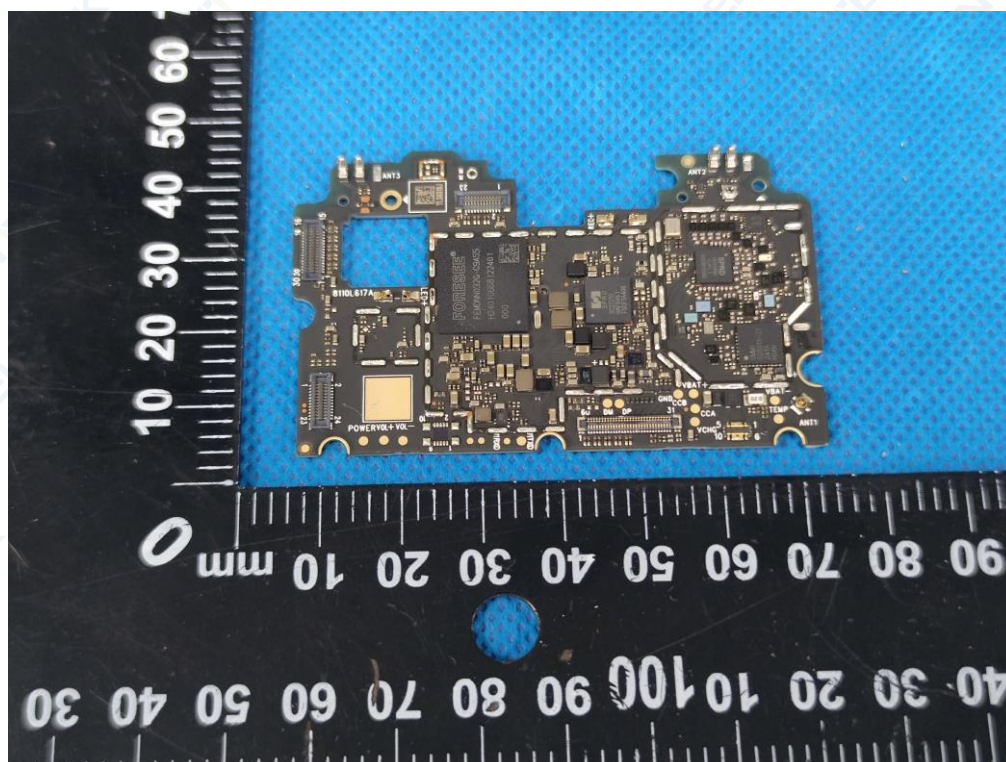
Figure 14 PCB view
