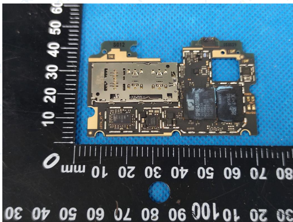
Figure 13 PCB view
