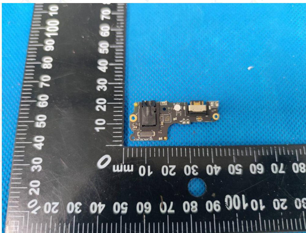
Figure 11 PCB view
