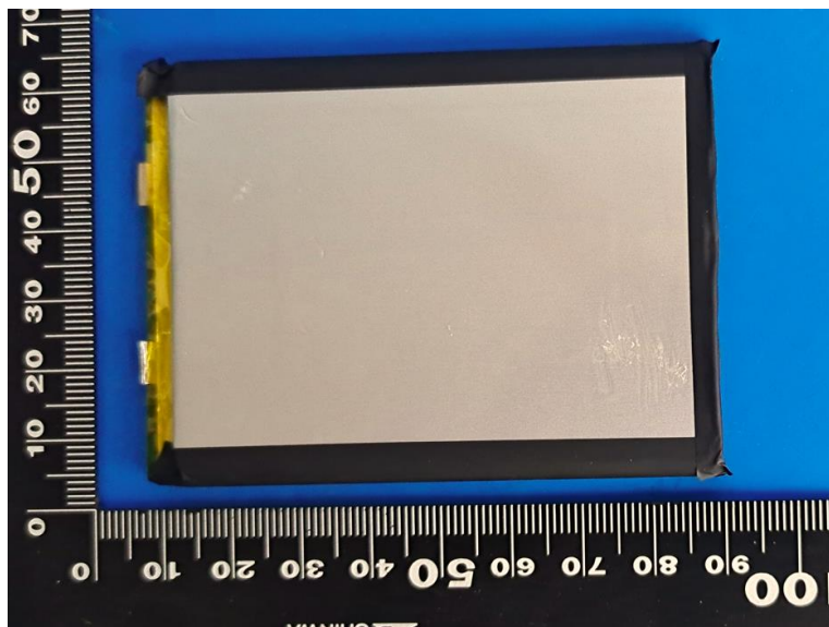
Fig. 4 – Back view of Cell 表4 –电芯反面视图
