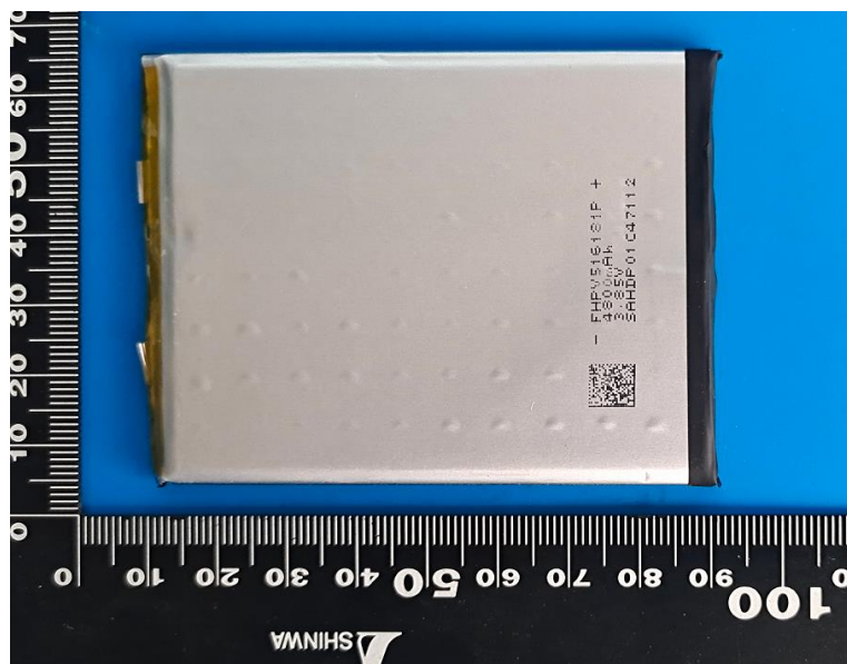
Fig. 3 – Front view of Cell 表3 –电芯正面视图
