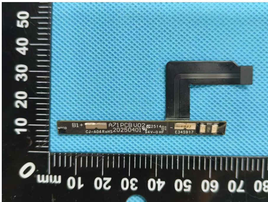
Fig.6- Back view of PCB
