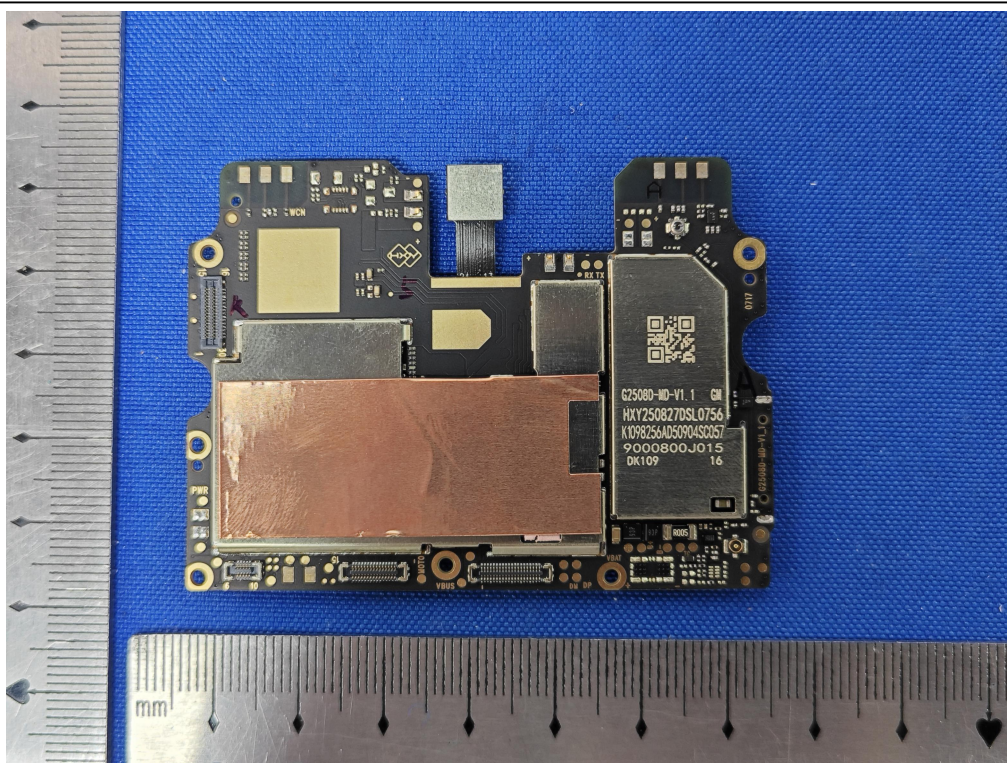
Photo 9 PCB view
