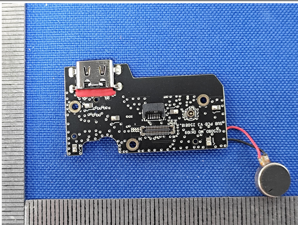
Photo 11 PCB view
