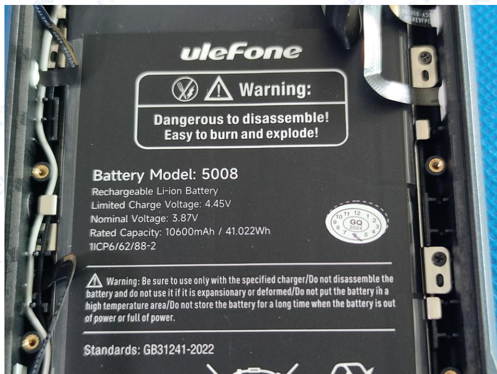
Figure 14 Battery view
