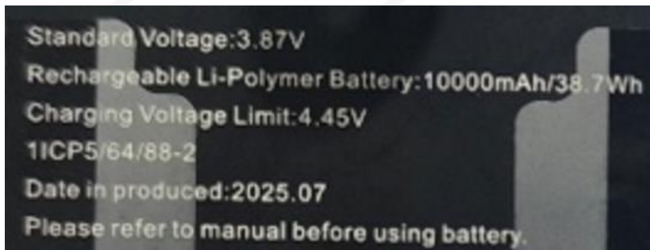
Figure 6 Label view of battery pack
