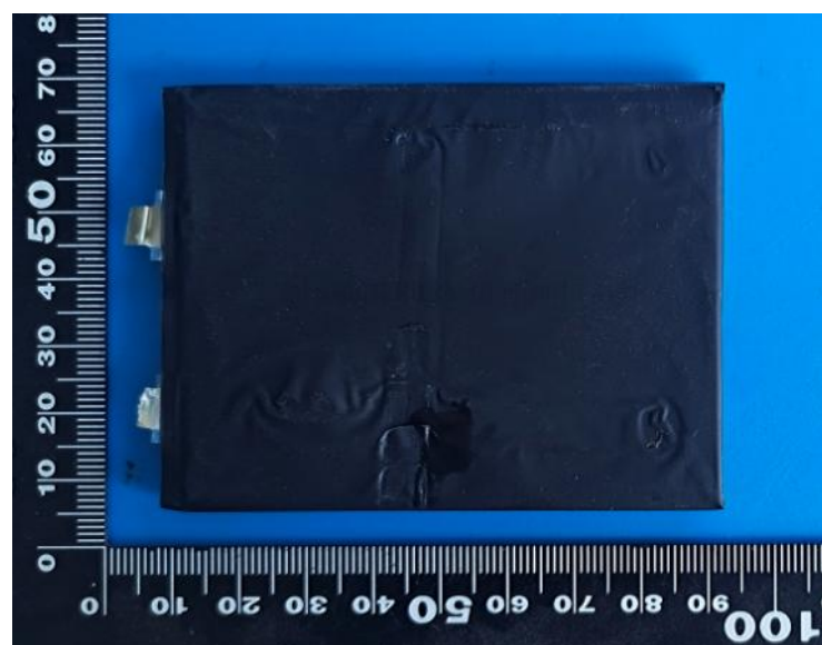
Fig. 4 – Back view of Cell 表4 – 电芯反面视图
