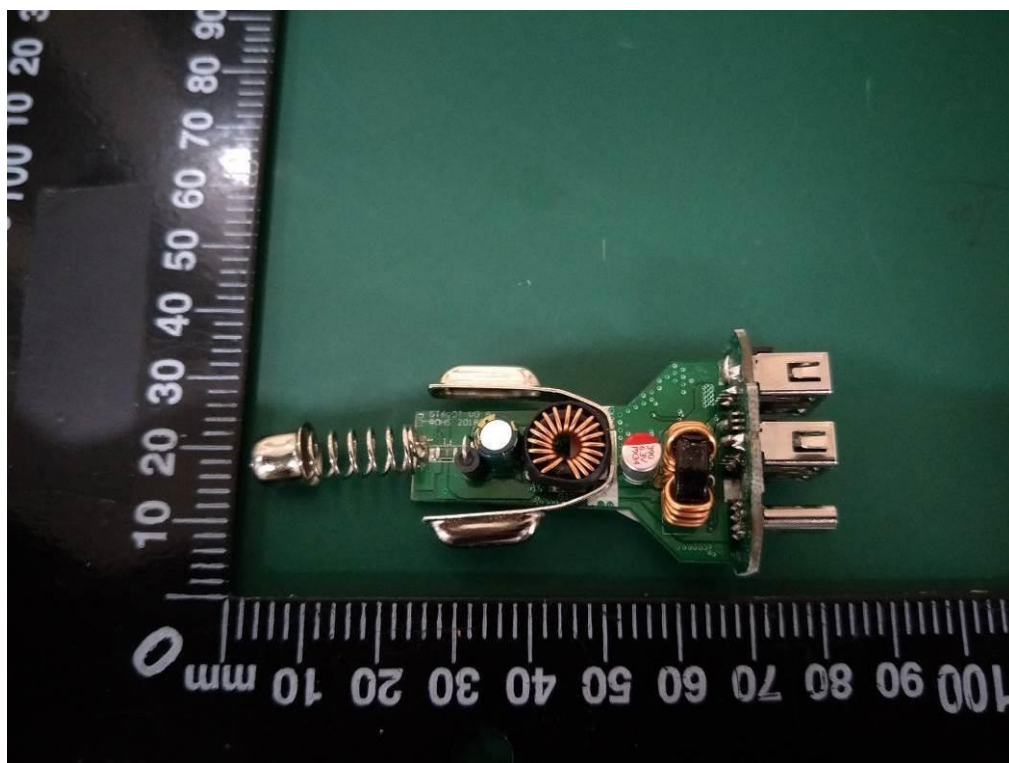
Figure 4.View of PCB
