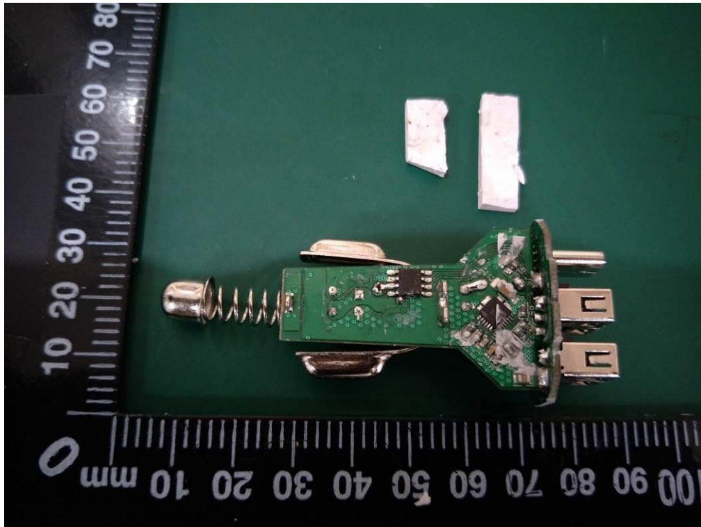
Figure 5.View of PCB
