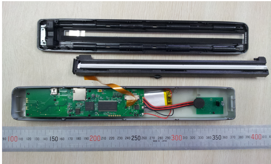
FIGURE 3 Inside of EUT(M/N: iScan02)
