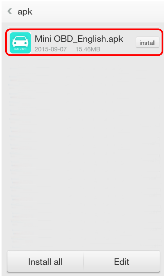
Andriod Software
