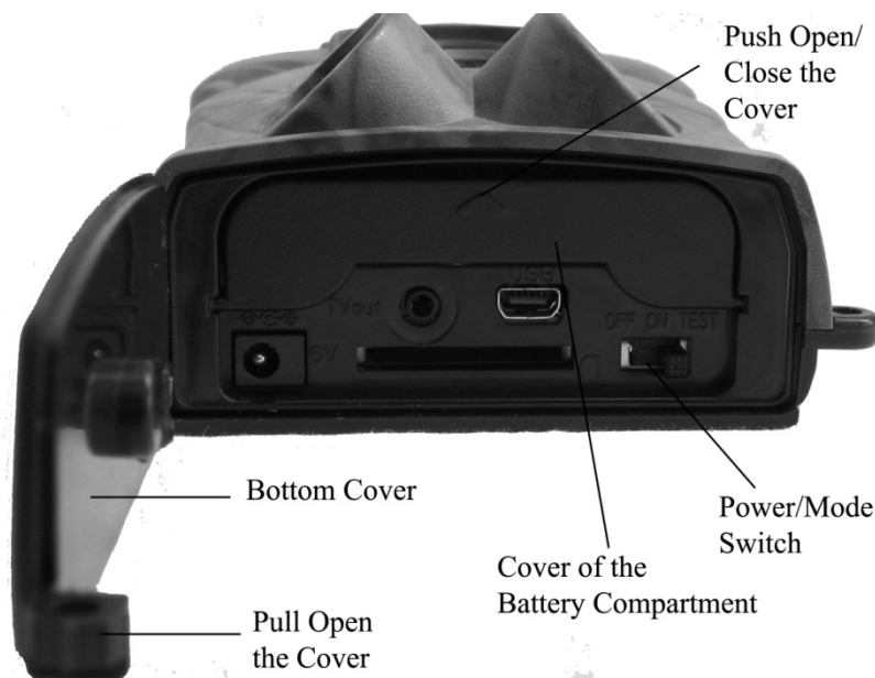
Figure 1.2: Bottom View
