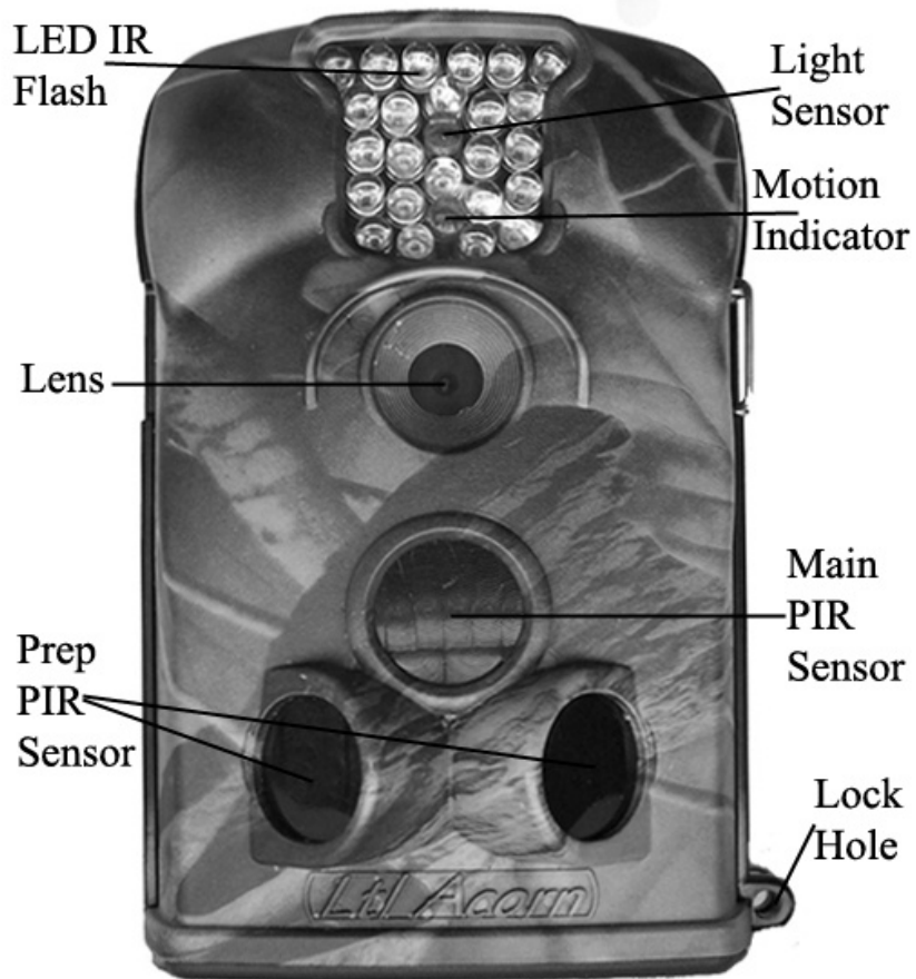
Figure 1.1: Front View
