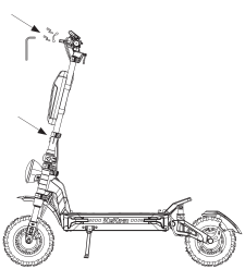
3.Tighten the handlebar fixing clamp block with screws, install the handlebar and hanging bag, and start the machine for inspection.
