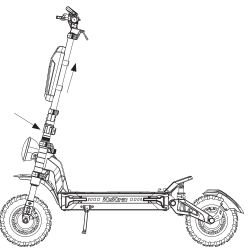
2.Loosen the locking buckle and pull the body rod upwards.
